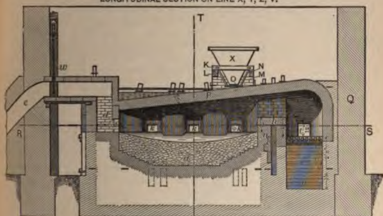
Fig. 28 LONGITUDINAL SECTION ON LINE X, Y, Z, V.
